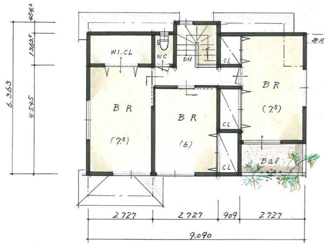
2F PLAN
